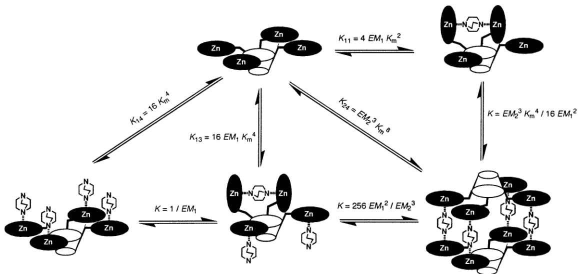
Figure 12. Equilibria present in mixtures of 1 and DABCO. EM_1 and EM_2 are the effective molarities for the intramolecular interactions required to form the intramolecular and intermolecular sandwich complexes 1 \cdot \text{DABCO} and (1)_2 \cdot (\text{DABCO})_4 , respectively. K_m is the microscopic association constant for the interaction of one DABCO nitrogen with a zinc porphyrin. Stepwise equilibrium constants ( K ), overall stability constants ( K_{11} , K_{24} , K_{13} , and K_{14} ), and statistical correction factors for the equilibria are also shown.
