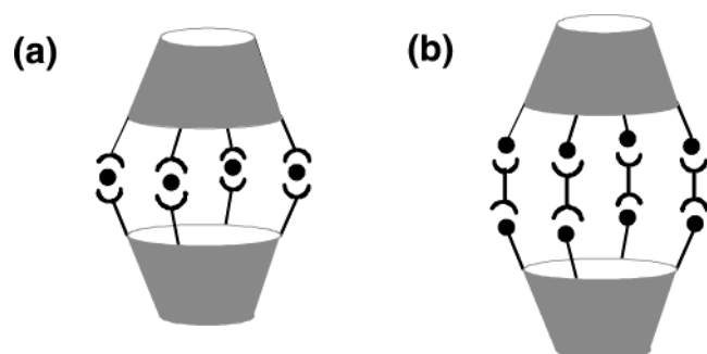
Figure 1. Dalcanale's resorcinarene dimer is assembled via coordination of four metals (●). (b) The strategy employed here is assembly of a calixarene bearing four metal centers (●) via coordination of four bidentate ligands.
