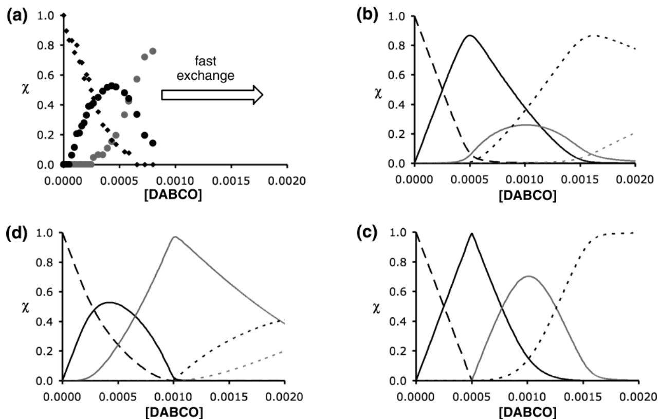
Figure 10. ^1\text{H} NMR titration of 1 (0.5 mM) with DABCO in \text{CDCl}_3 at 295 K. (a) Experimental data for the mole fraction ( X ) of free 1 ( \blacklozenge ), the 1:1 stoichiometry 1 -DABCO complex ( \bullet ), and the 1:2 stoichiometry 1 -DABCO complex (gray circle). (b) Simulated concentration profiles for binding Model 3 showing the mole fraction of free 1 (---), 1 -DABCO (-), 1 -(DABCO) _2 (gray line), 1 -(DABCO) _3 (- - -), and 1 -(DABCO) _4 (gray dashed line). (c) Simulated concentration profiles for binding Model 4 showing the mole fraction of free 1 (---), ( 1 ) _2 -(DABCO) _2 (-), ( 1 ) _2 -(DABCO) _4 (gray line), ( 1 ) _2 -(DABCO) _6 (- - -), and 1 -(DABCO) _4 (gray dashed line) which does not appear in this concentration range. (d) Simulated concentration profiles for binding Model 5 showing the mole fraction of free 1 (---), 1 -DABCO (-), ( 1 ) _2 -(DABCO) _4 (gray line), 1 -(DABCO) _3 (- - -), and 1 -(DABCO) _4 (gray dashed line).
