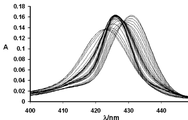
Figure 9. UV-visible titration of 1 (0.1 \mu M) with DABCO in CH 2 Cl 2 at 295 K.
