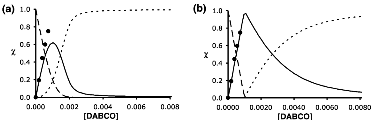
Figure 8. 1 H NMR titration of 9 (1 mM) with DABCO in CDCl 3 at 295 K. (a) Simulated concentration profiles for the intramolecular sandwich model shown in Figure 6a, showing the mole fraction of free 9 (---), 9 ·DABCO (—), and 9 ·(DABCO) 2 (· · ·). (b) Simulated concentration profiles for the intermolecular sandwich model shown in Figure 6b, showing the mole fraction of free 9 (---), ( 9 ) 2 ·(DABCO) 2 (—), and 9 ·(DABCO) 2 (· · ·). The experimental mole fraction ( \chi ) of sandwich complex (●) determined by integration of 1 H NMR signals in the slow exchange phase of the titration is shown for comparison.
